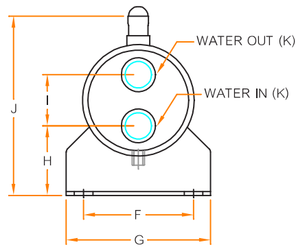
FIXED SUPPORT
